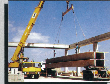
Erection of Prestressed TT-Beams
