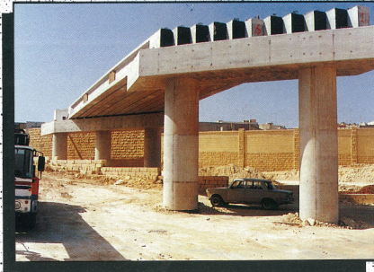
Prestressed Bridge Beams at St. Venera Viaduct
