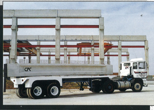
Prestressed I-Beams
