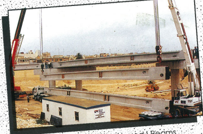
Erection of Long-Span Prestressed I-Beams
